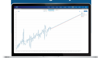
Trending analysis
