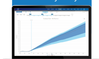
Uncertainty analysis
